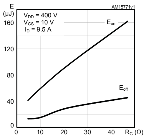
Figure 13. Typical switching energy vs gate resistance
