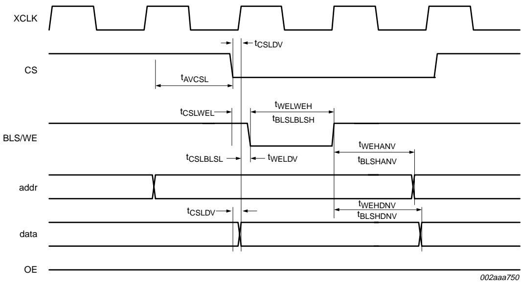
Fig 6. External memory write access
