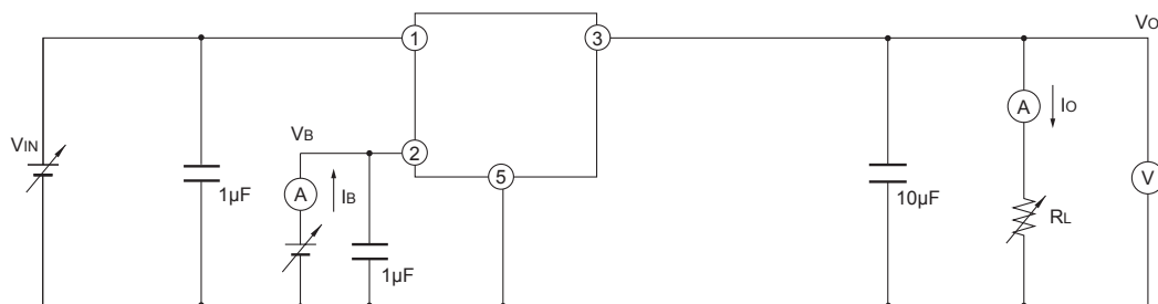
Fig.1 Test Circuit
