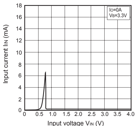
Fig.26 Input Current vs. Input Voltage (PQ008GN01ZPH)
