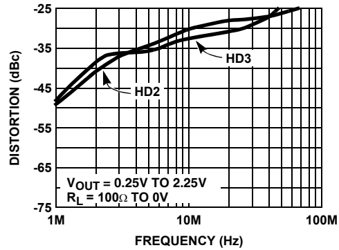
FIGURE 33. 2nd AND 3rd HARMONIC DISTORTION vs FREQUENCY
