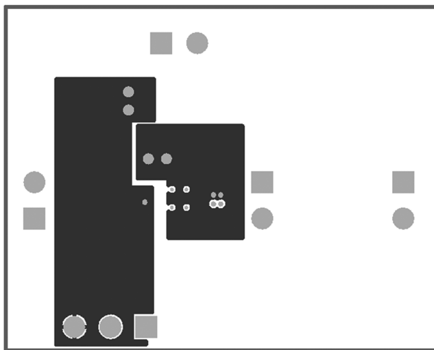
Bottom Silkscreen
