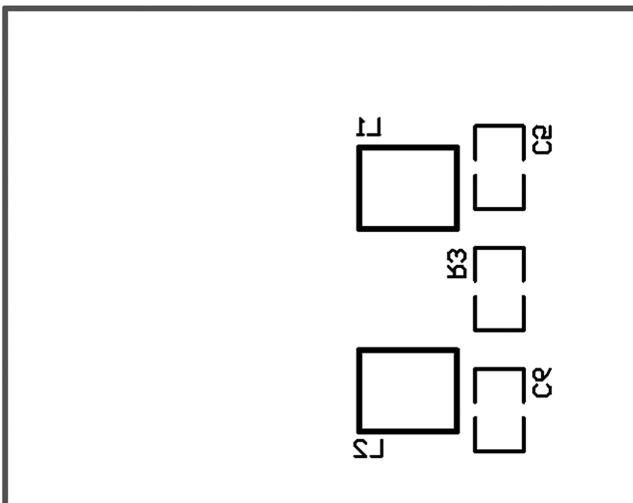
Bottom Silkscreen
