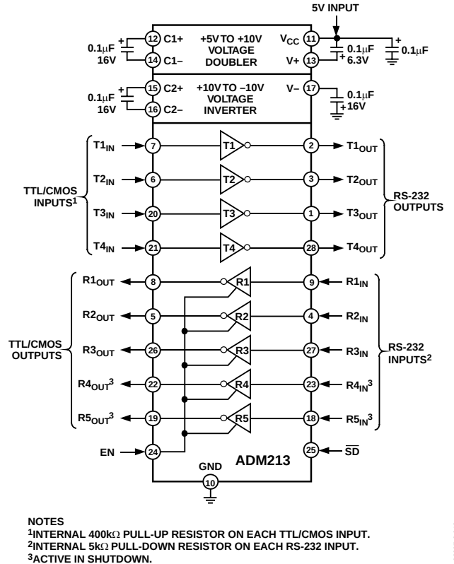
Figure 13. ADM213 Typical Operating Circuit
