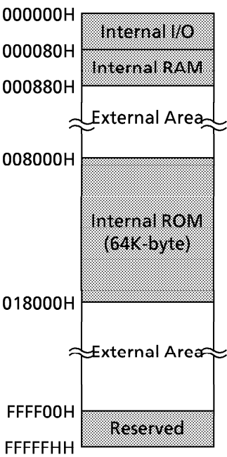
Fig.1.1 Memory map of TMP93CS40 / PS40
