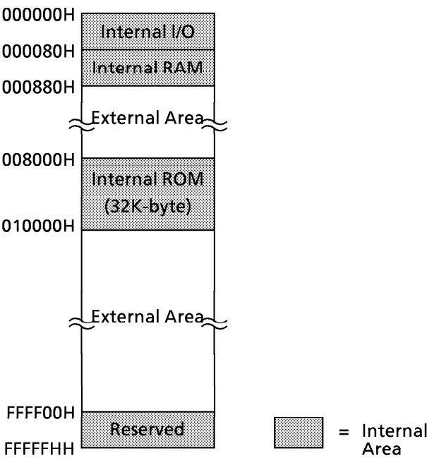
Fig.1.2 Memory map of TMP93CM40
