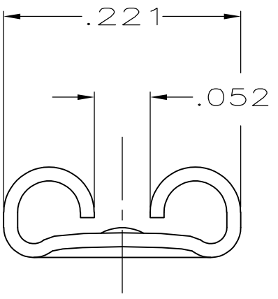
VIEW X-X SCALE 8:1
