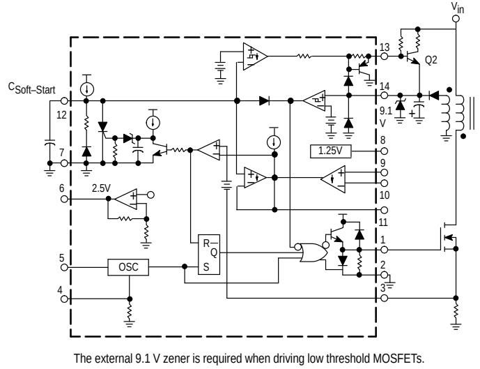
Figure 21. Bootstrap Startup
