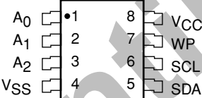
TSSOP Package (U, Y, GY)
