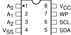
TSSOP Package (U, Y, GY)
