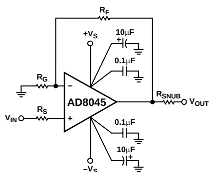
Figure 61. Noninverting Configuration
