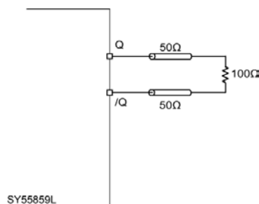
Figure 6. Output Interface
