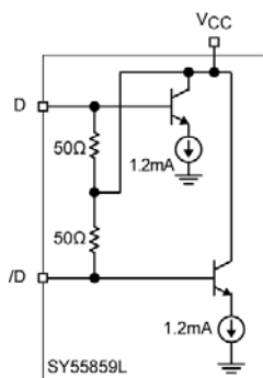
Figure 1. Input Structure
