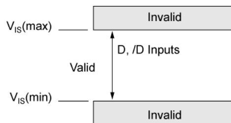
Figure 4. Input Range
