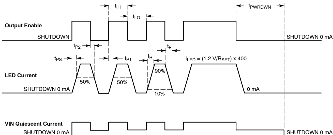
Figure 2. CAT4109/CAV4109 OE Timing
