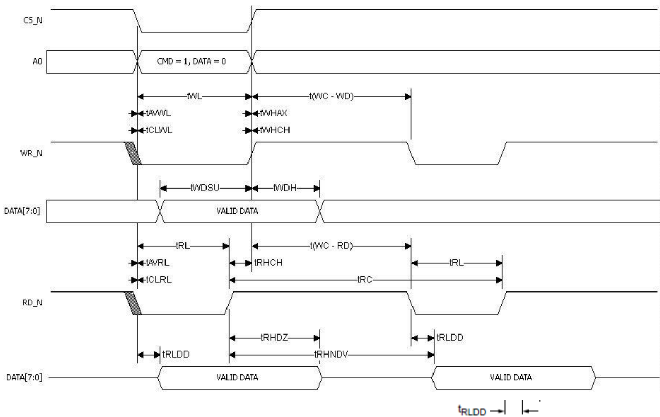
Figure 8-2 Parallel interface timing
