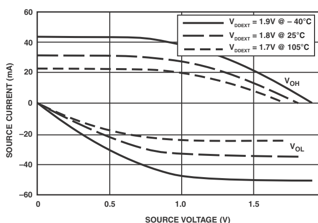
Figure 51. Driver Type D Current ( 1.8V V_{DDEXT}/V_{DDMEM} )
