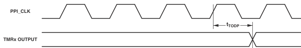
Figure 30. Timer Clock Timing
