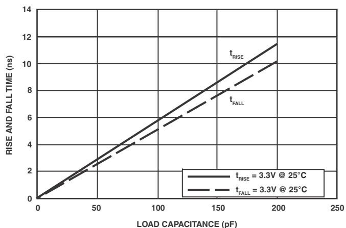
Figure 66. Driver Type C Typical Rise and Fall Times (10%–90%) vs. Load Capacitance ( 3.3V_{DDEXT}/V_{DDMEM} )
