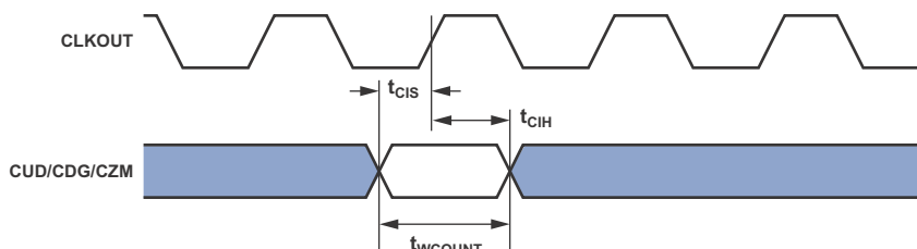
Figure 32. Up/Down Counter/Rotary Encoder Timing
