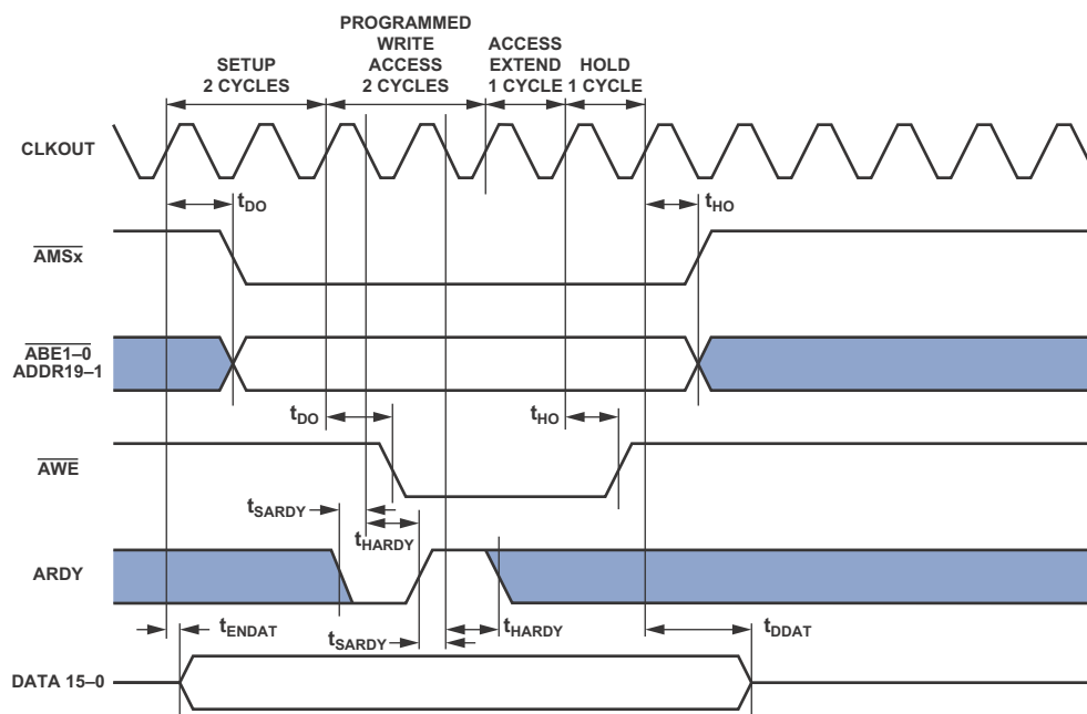
Figure 13. Asynchronous Memory Write Cycle Timing
