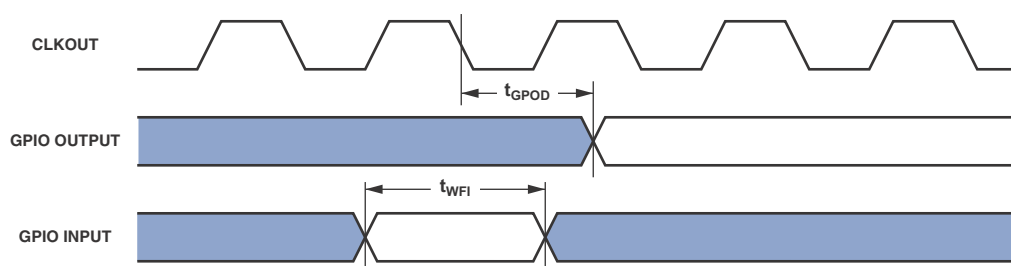
Figure 29. General-Purpose Port Timing
