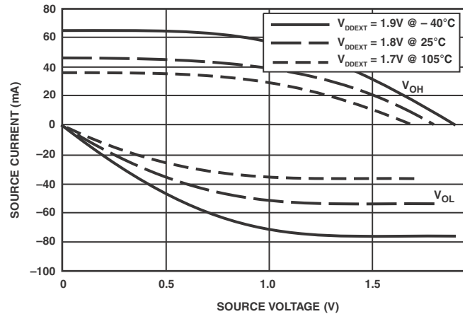
Figure 45. Driver Type B Current ( 1.8V_{DDEXT}/V_{DDMEM} )
