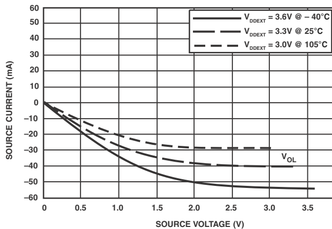
Figure 52. Driver Type E Current ( 3.3V_{DDEXT}/V_{DDMEM} )
