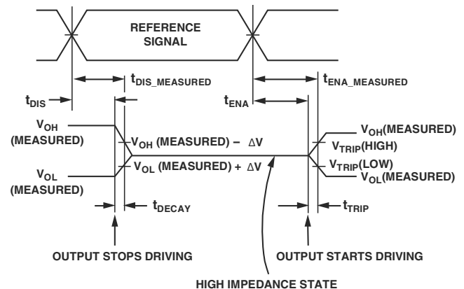
Figure 56. Output Enable/Disable
