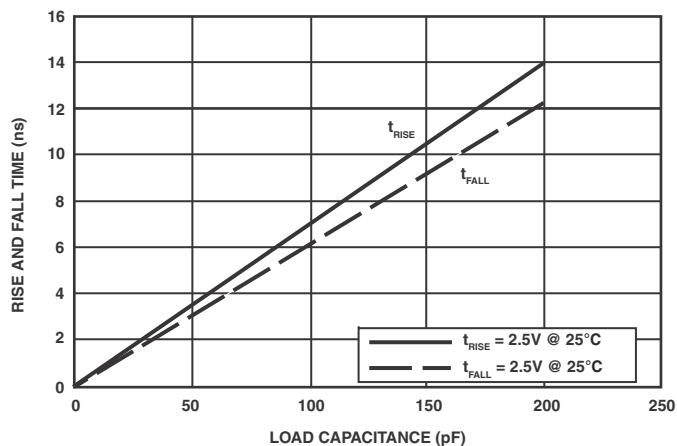
Figure 65. Driver Type C Typical Rise and Fall Times (10%–90%) vs. Load Capacitance ( 2.5V_{DDEXT}/V_{DDMEM} )
