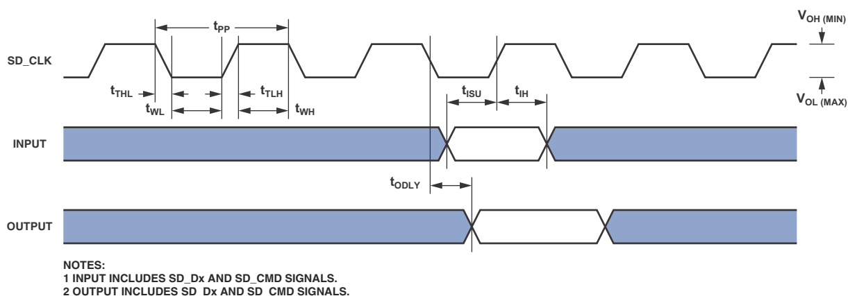
Figure 21. RSI Controller Timing
