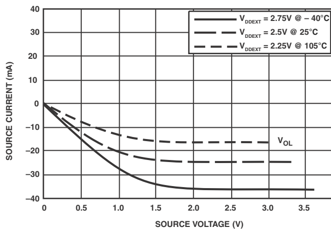
Figure 53. Driver Type E Current ( 2.5V_{DDEXT}/V_{DDMEM} )
