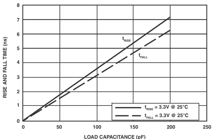
Figure 69. Driver Type D Typical Rise and Fall Times (10%–90%) vs. Load Capacitance ( 3.3V_{DDEXT}/V_{DDMEM} )
