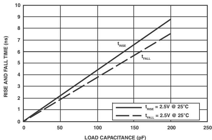
Figure 68. Driver Type D Typical Rise and Fall Times (10%–90%) vs. Load Capacitance ( 2.5V_{DDEXT}/V_{DDMEM} )
