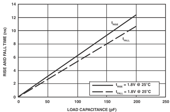
Figure 67. Driver Type D Typical Rise and Fall Times (10%–90%) vs. Load Capacitance ( 1.8V_{DDEXT}/V_{DDMEM} )
