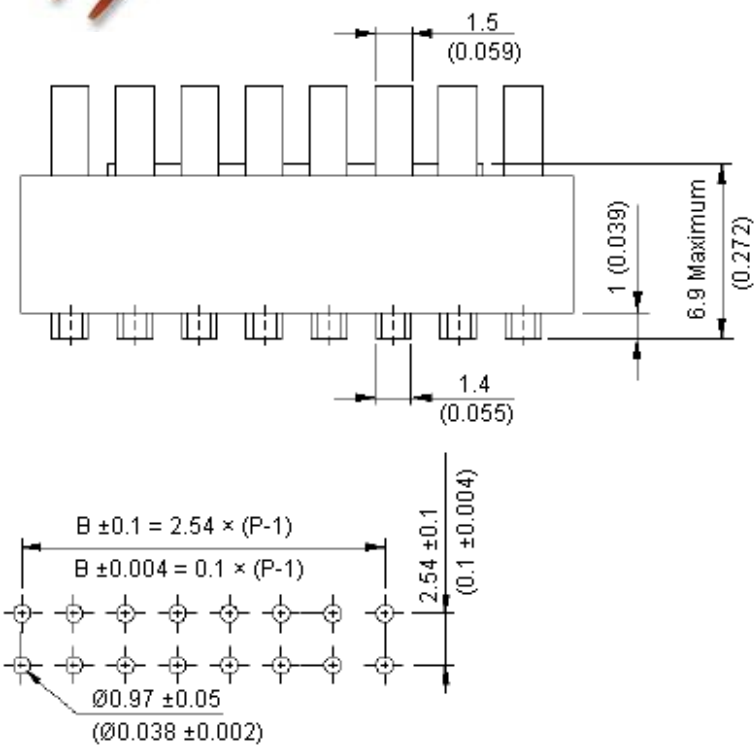
PCB Layout
