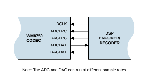
Figure 13 Slave Mode
