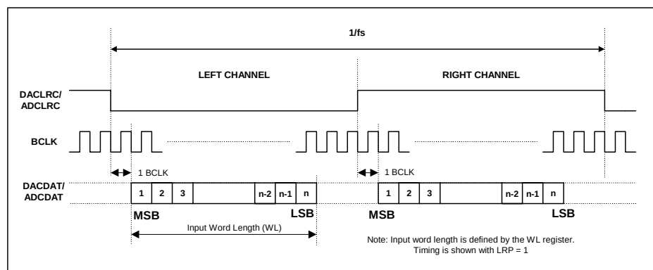
Figure 16 I 2 S Justified Audio Interface (assuming n-bit word length)
