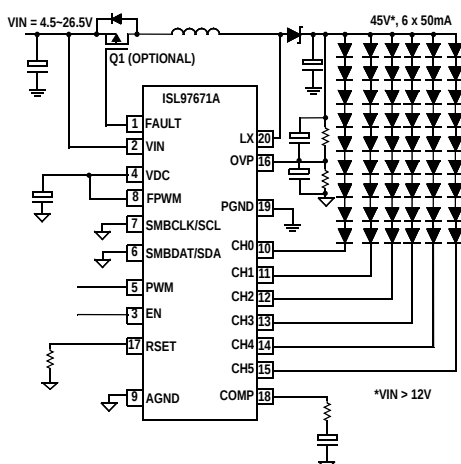
FIGURE 1C. DIRECT PWM DIMMING
