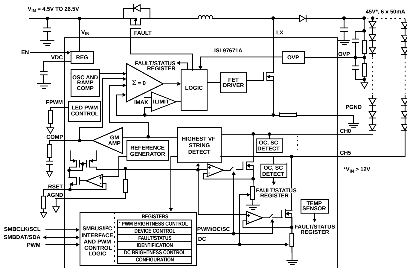
FIGURE 2. ISL97671A BLOCK DIAGRAM
