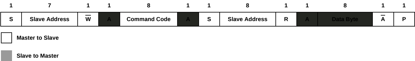
FIGURE 27. READ BYTE PROTOCOL
