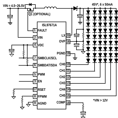
FIGURE 1A. SMBus/I 2 C CONTROLLED DIMMING AND ADJUSTABLE DIMMING FREQUENCY
