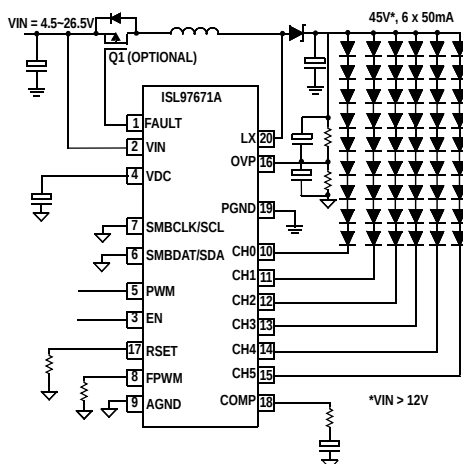
FIGURE 1B. PWM DIMMING WITH PWM INPUT AND ADJUSTABLE DIMMING FREQUENCY
