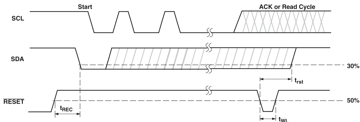
Figure 2. Reset Timing
