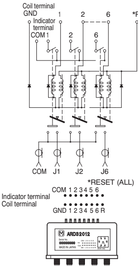
Latching type
