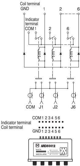
Fail-safe type
