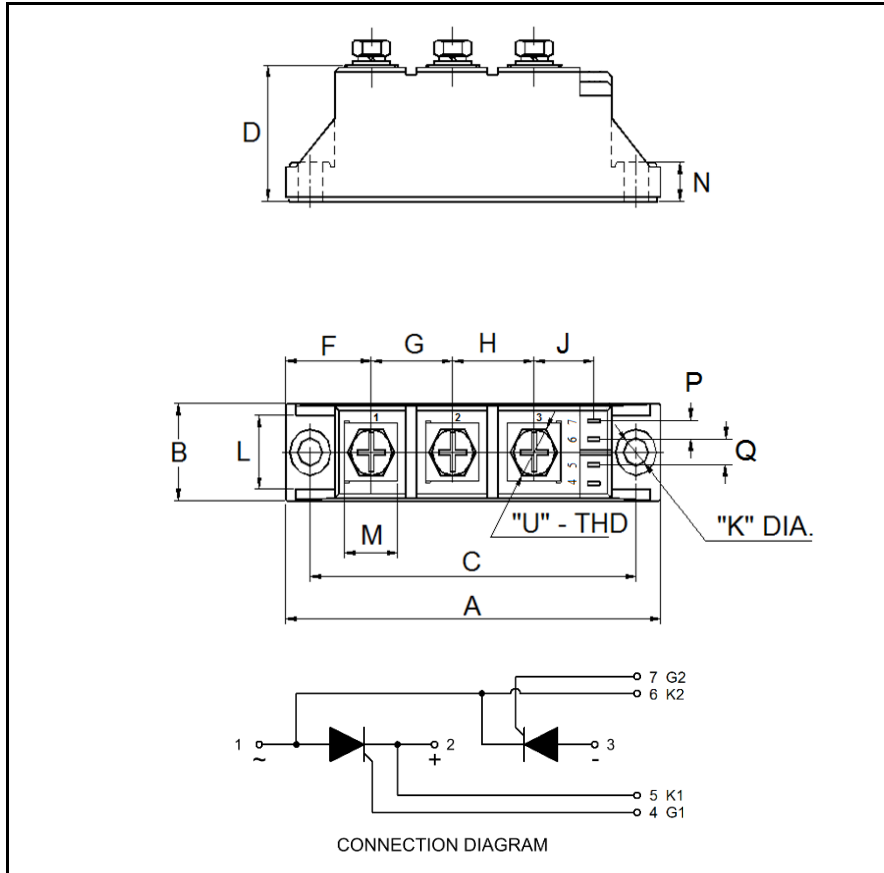
CD43__99C Dual SCR Isolated POW-R-BLOK™ Module 100 Amperes / Up to 1800 Volts
