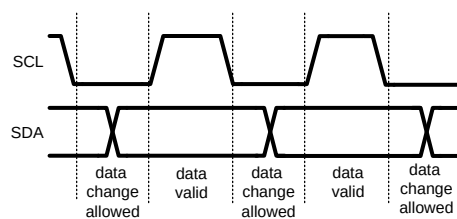
Figure 24. I 2 C Signals: Data Validity
