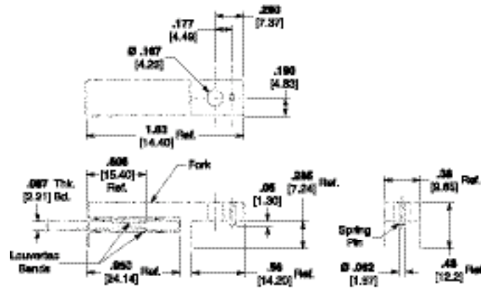
Part Number 194305-1
