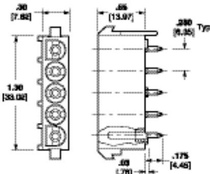
5 Circuit Part No. 194018-1
