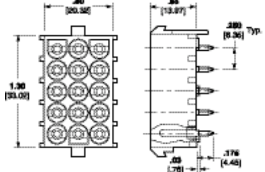
15 Circuit Part No. 194013-1
