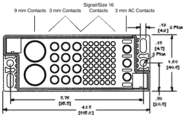
Receptacle 194069-1 (shown) 194069-3 with two 6-32 inserts (Front Mounted)
