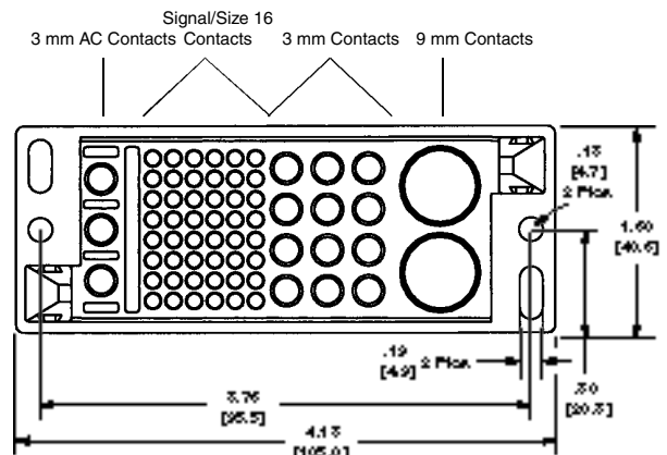
Plug 194070-1 (shown) 194070-3 with two 6-32 inserts (Front Mounted)
