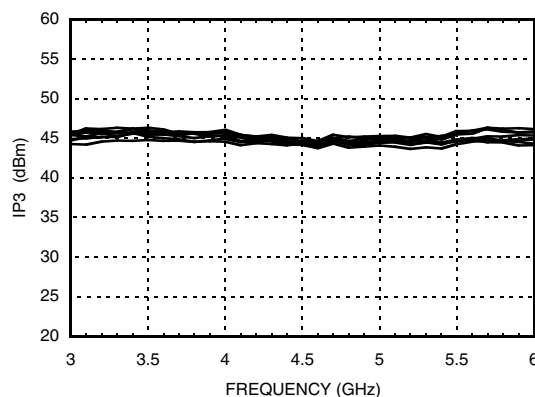
Input IP3, Major States Only
