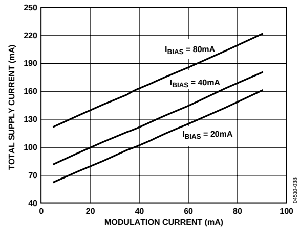
Figure 15. Total Supply Current vs. Modulation Current \text{Total Supply Current} = I_{CC} + I_{bias} + I_{mod}
