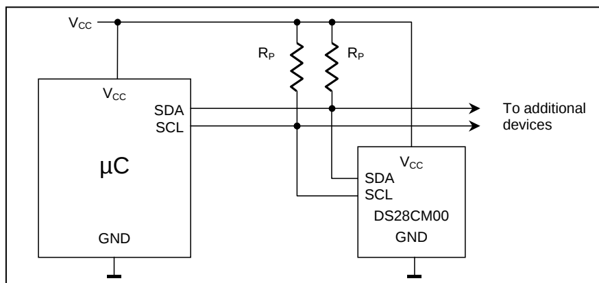
Figure 6. Application Schematic
