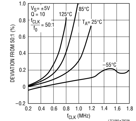
Graph 9. Mode 1: ( f_{CLK}/f_0 ) vs f_{CLK} and Temperature
