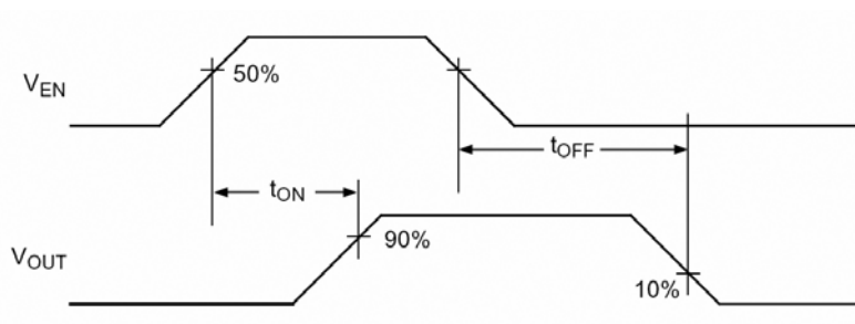
Figure 1a. MIC2544/48-1
