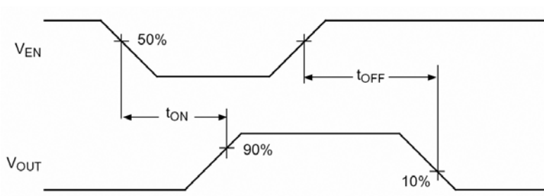
Figure 1b. MIC2544/48-2
