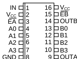
DS1045S 16-Pin SOIC (300-mil) See Mech. Drawings Section
