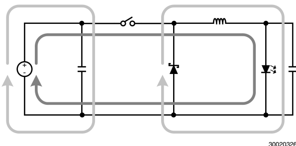
FIGURE 11. Buck Converter Current Loops
