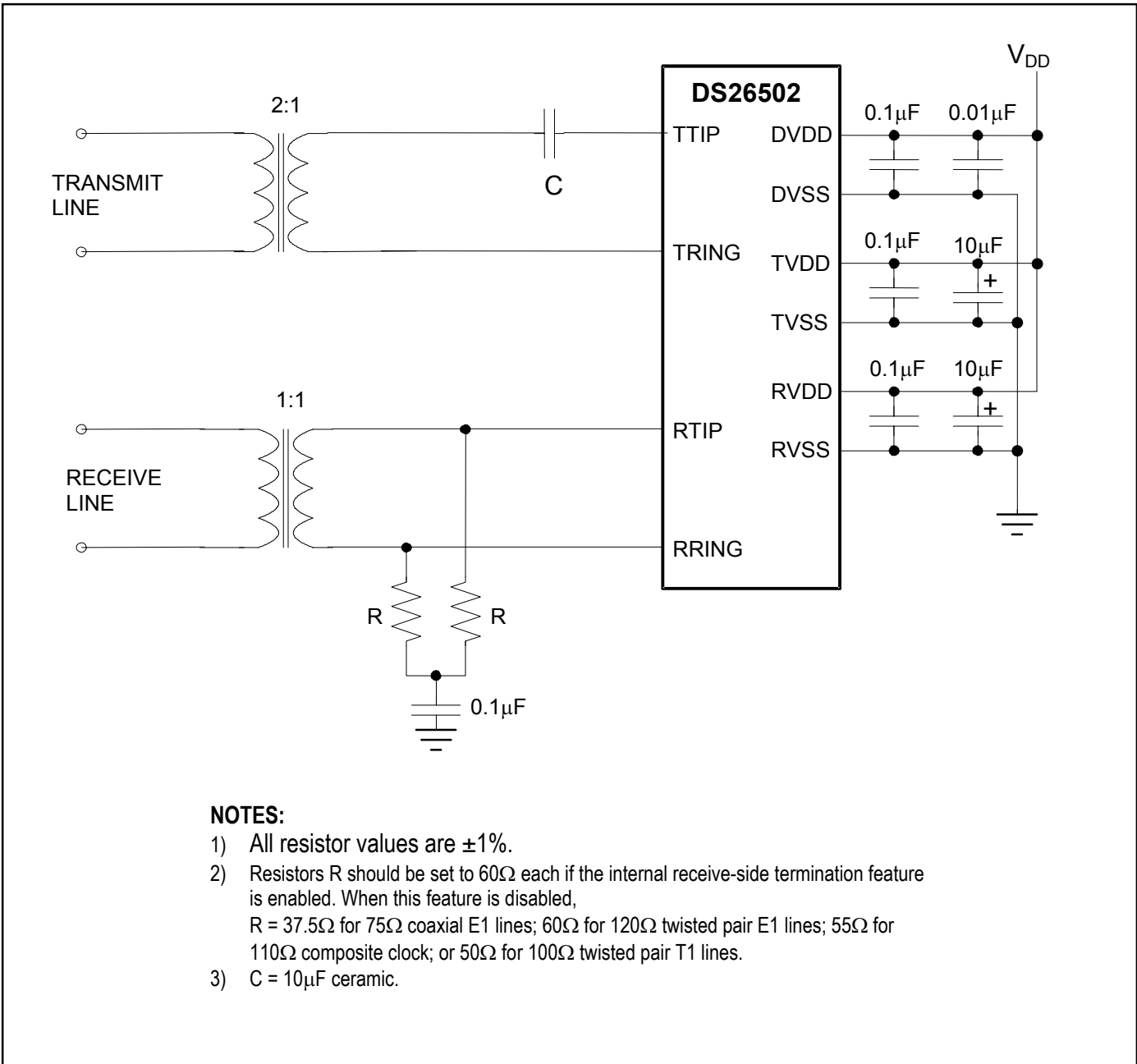
Figure 13-4. Basic Interface
