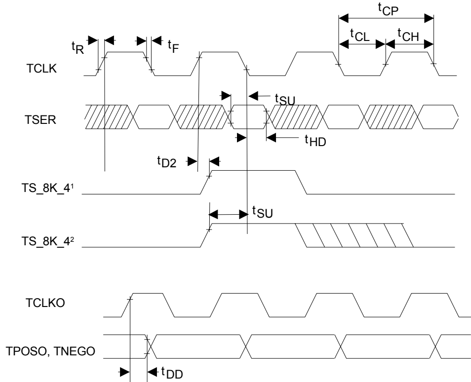
Figure 20-11. Transmit Timing, T1, E1, 64KCC Mode
