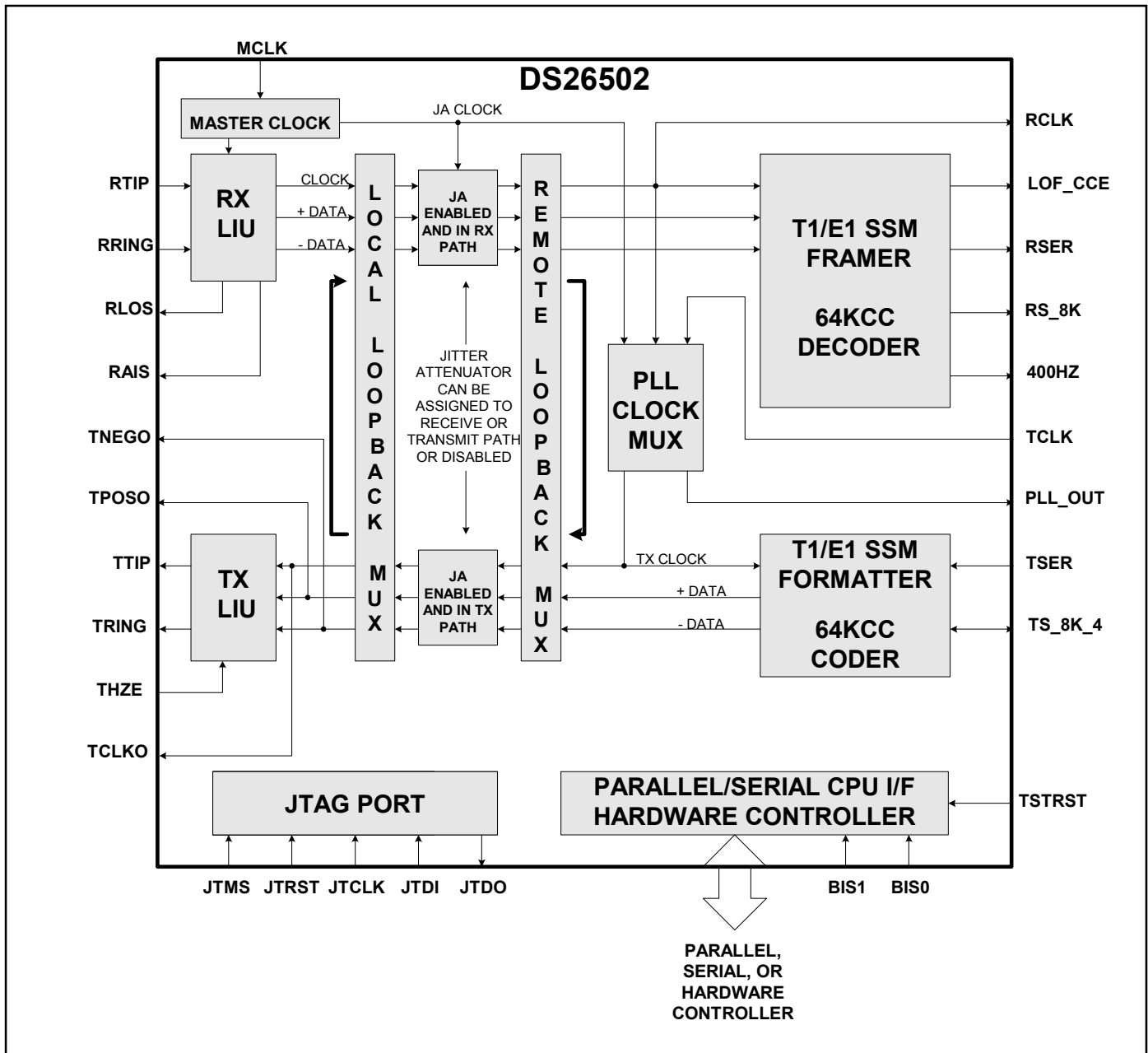
Figure 3-1. Block Diagram
