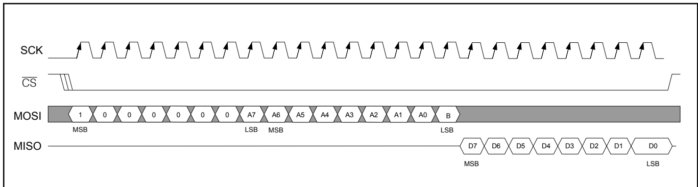
Figure 18-1. SPI Serial Port Access, Read Mode, CPOL = 0, CPHA = 0
