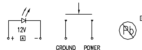
INTERNAL CIRCUIT
