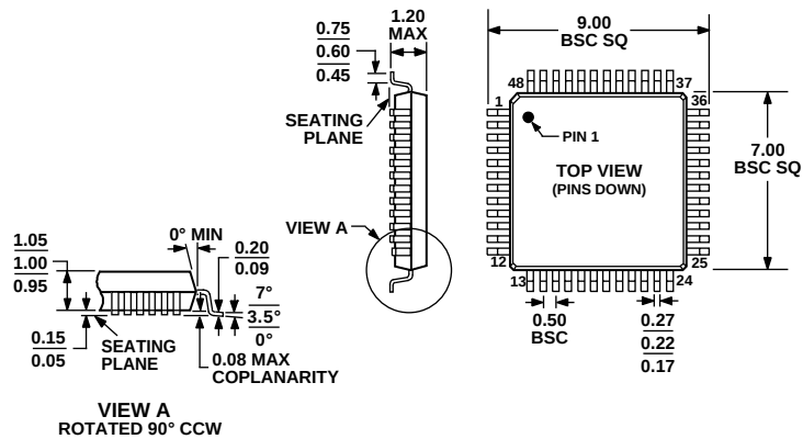
Figure 43. 48-Lead Thin Plastic Quad Flat Package [TQFP] (SU-48) Dimensions shown in millimeters
