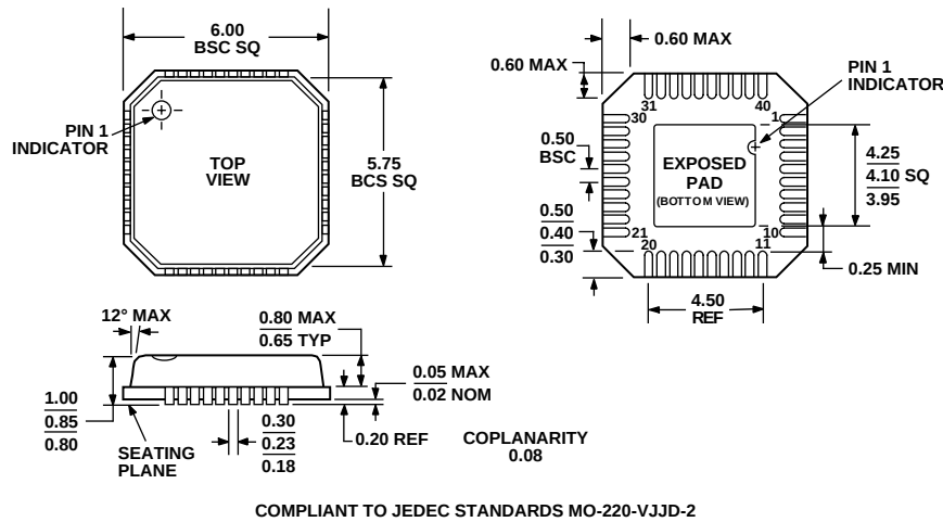
Figure 42. 40-Lead Lead Frame Chip Scale Package [LFCSP] (CP-40) Dimensions shown in millimeters
