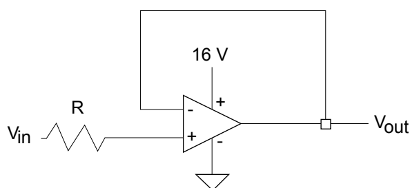
Figure 26. Input current limitation
