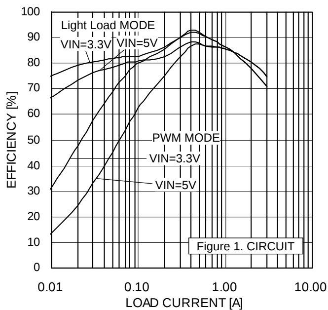
Figure 8. Efficiency(BD90535EFJ-C)
