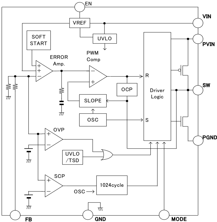
Figure 4. Block diagram
