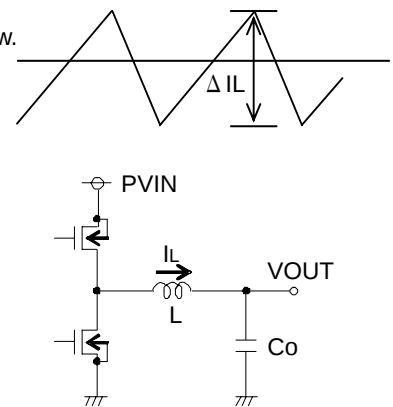
Figure 30. Ripple current
