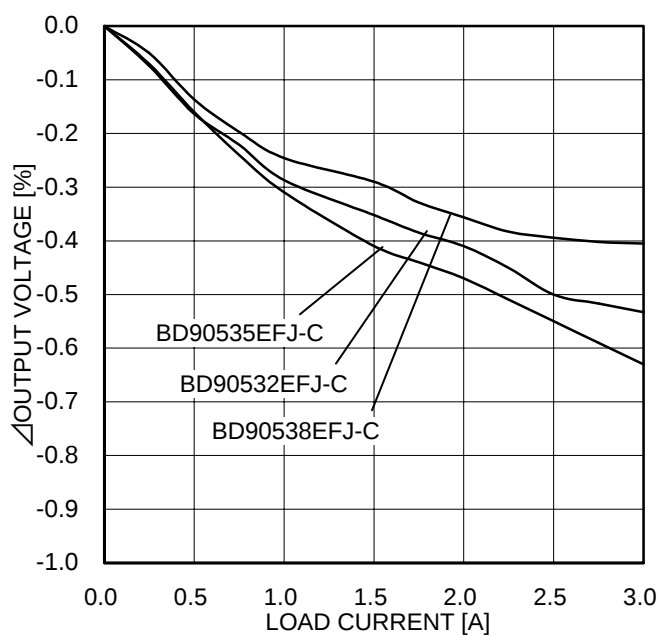
Figure 15. Load regulation
