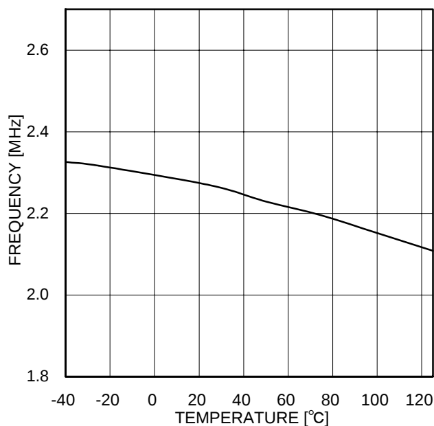
Figure 18. Frequency vs. temperature
