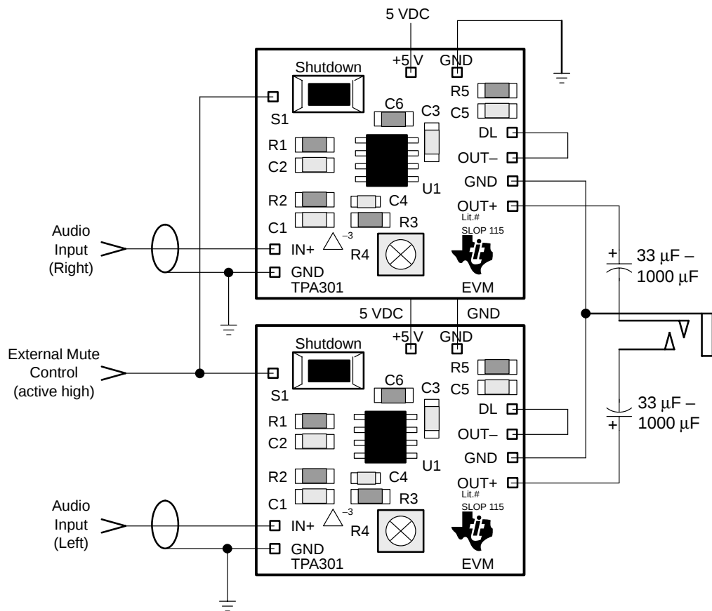
Figure 3–9. TPA301 EVM Connected for Stereo Single-Ended Output
