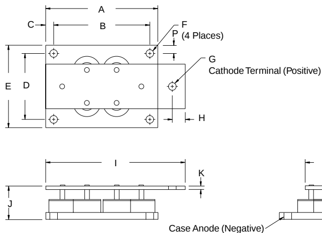
GPZ1275 PACKAGE OUTLINE
