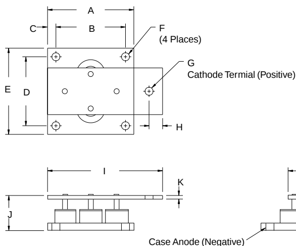
GPZ532 PACKAGE OUTLINE
