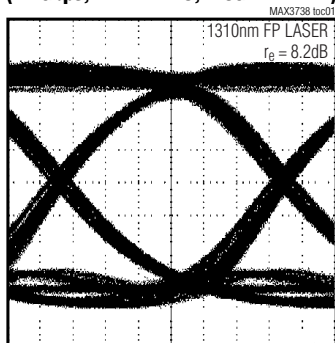
OPTICAL EYE DIAGRAM (2.7Gbps, 2^7 - 1 PRBS, 2.36GHz FILTER)
