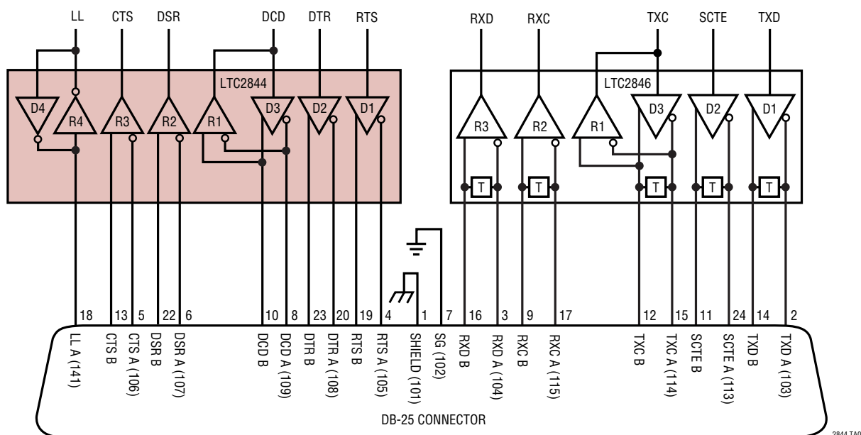
DTE or DCE Multiprotocol Serial Interface with DB-25 Connector
