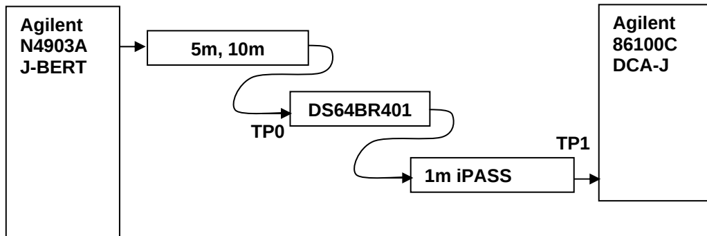
Figure 3. DS64BR401EVK Equalization Test Setup
