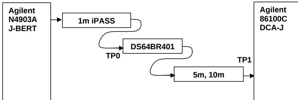
Figure 4. DS64BR401EVK De-emphasis Test Setup
