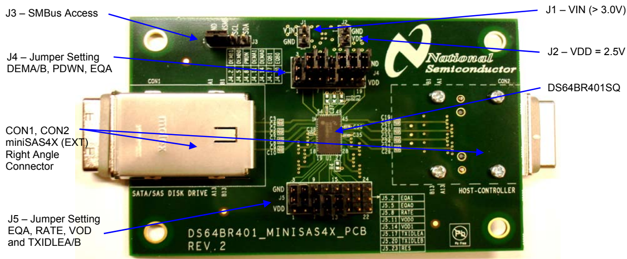
Figure 1. DS64BR401EVK Evaluation Board
