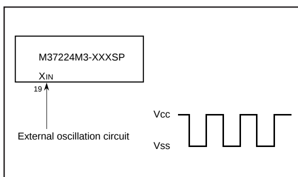
Fig. 56. External Clock Input Circuit Example
