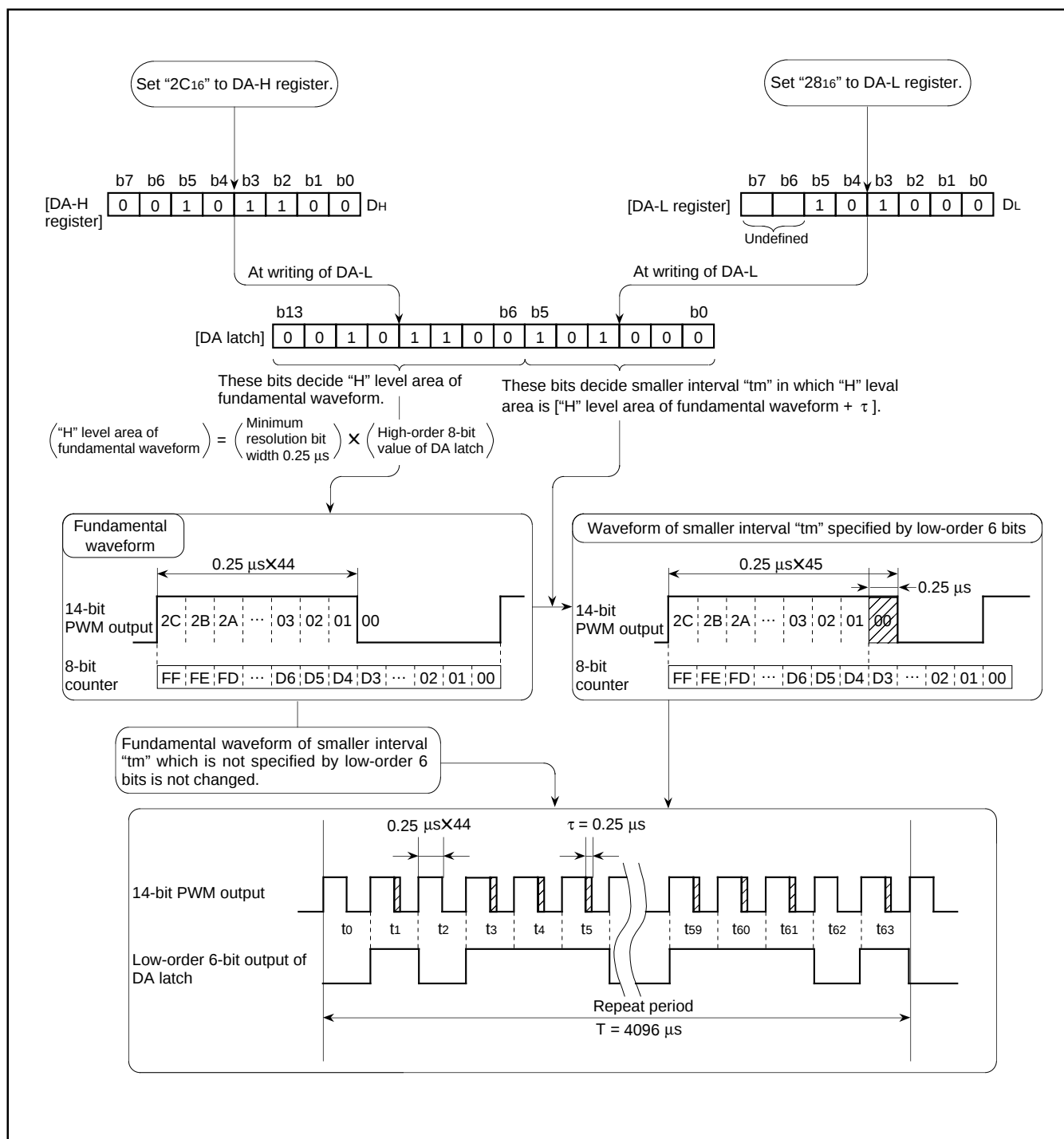
Fig. 24. 14-bit PWM Output Example ( f(X_{IN}) = 8 \text{ MHz} )
