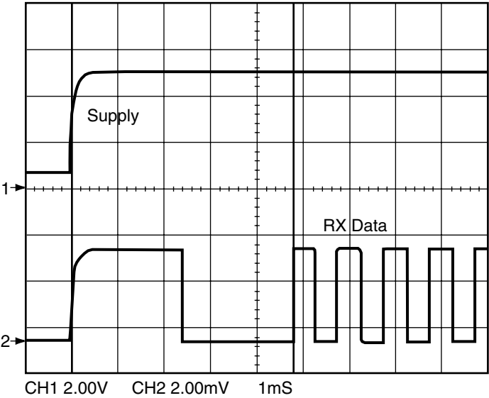
Figure 7: Rx V_{cc} to Valid Data
