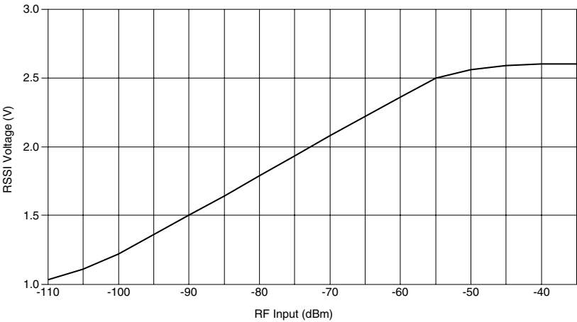
Figure 5: RSSI Characteristics Chart
