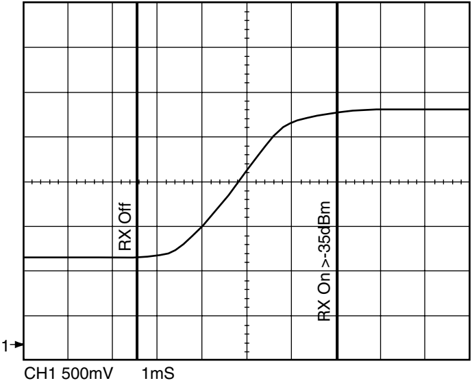
Figure 6: Worst Case RSSI Response Time
