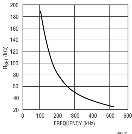
Figure 2. Timing Resistor ( R_{\text{SET}} ) Value
