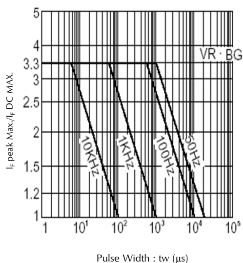
Pulse Width vs. Maximum Tolerable Peak Current Condition : T_a = 25
