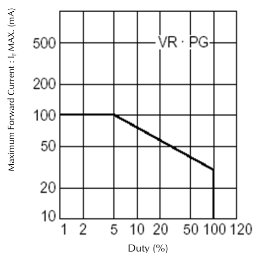
Dynamic Drive Rating Duty cycle vs. Maximum Forward Current Condition : Ta = 25
