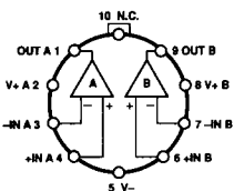
TO-100 (K-Suffix) OP-04
