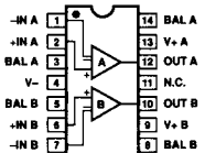
14-PIN HERMETIC DIP (Y-Suffix) OP-04
