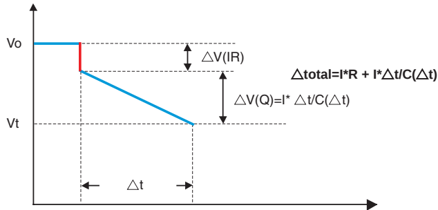
Figure 4. Voltage-time relation of capacitor unit
