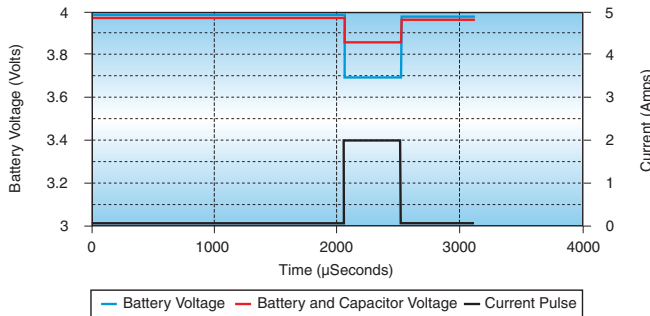
Figure 5. GSM Pulse
