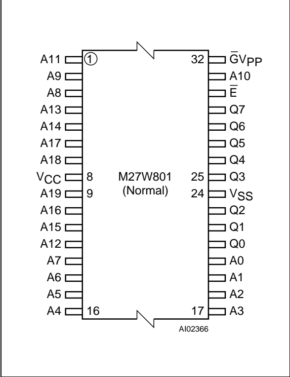
Figure 2C. TSOP Connections
