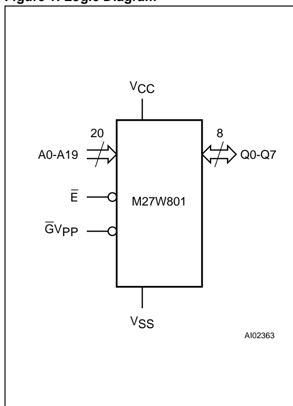
Figure 1. Logic Diagram
