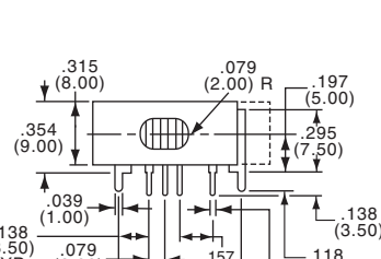
SP3T/DP3T
