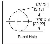
Panel Hole
