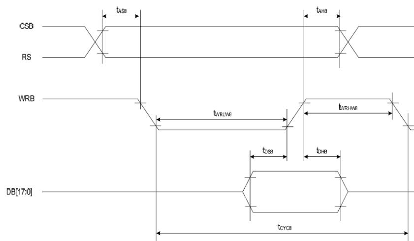
( Write Timing )
