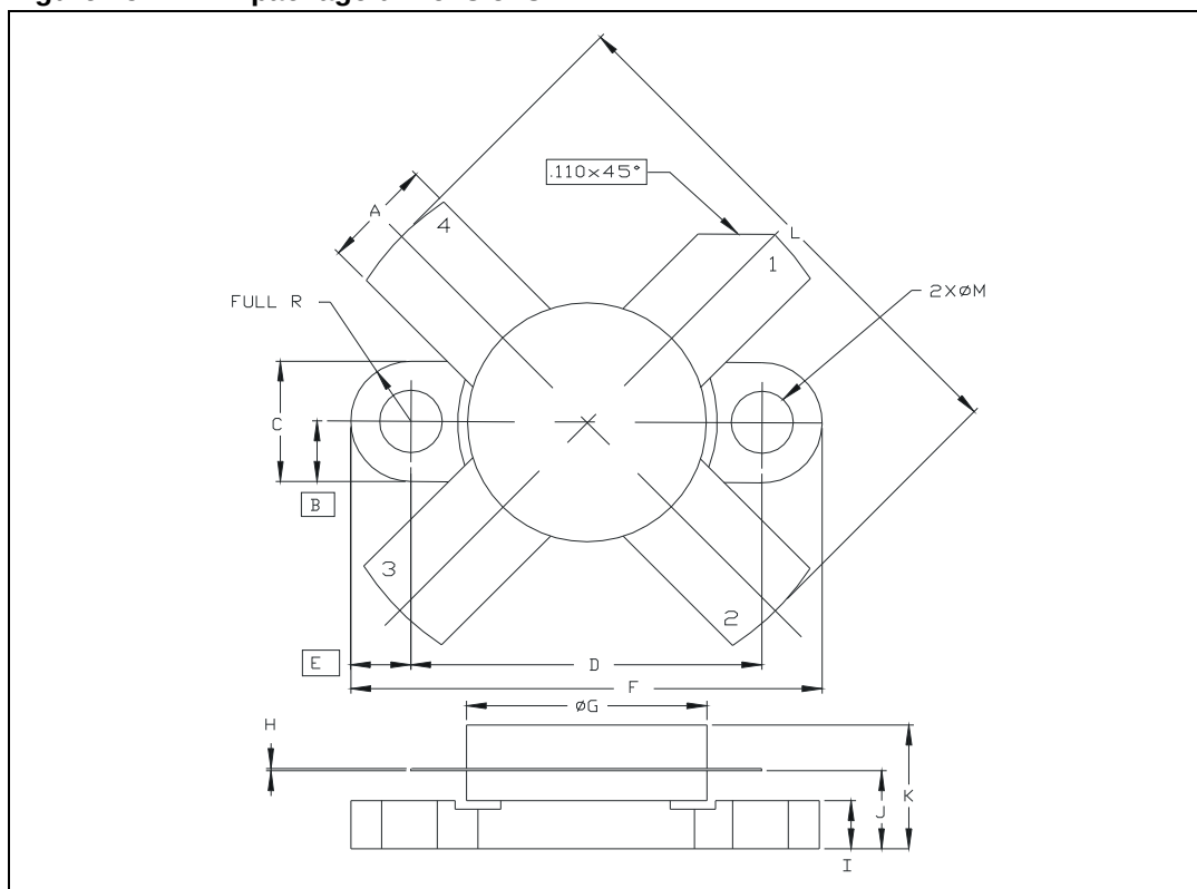
Figure 15. M174 package dimensions
